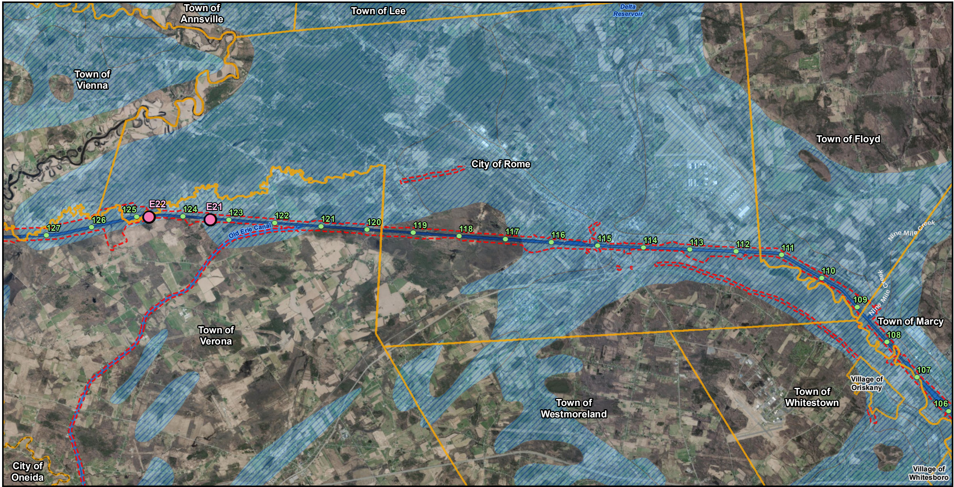
Figure 52F: Aquifers
